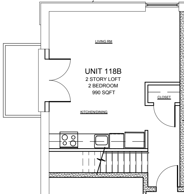
1 UNIT PLAN-LOWER LEVEL NOT TO SCALE
